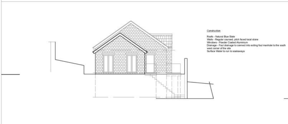
Plot 2 South Elevation
